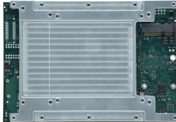
Heat spreader on bottom side
