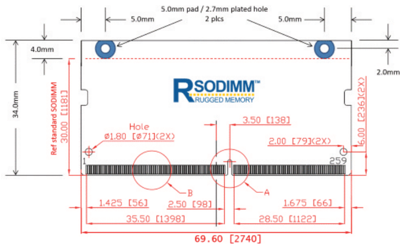
RSODIMM mechanical drawing
