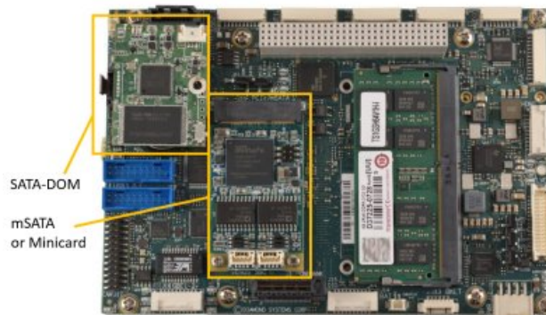
SATA-DOM and mSATA/minicard sockets on top side
